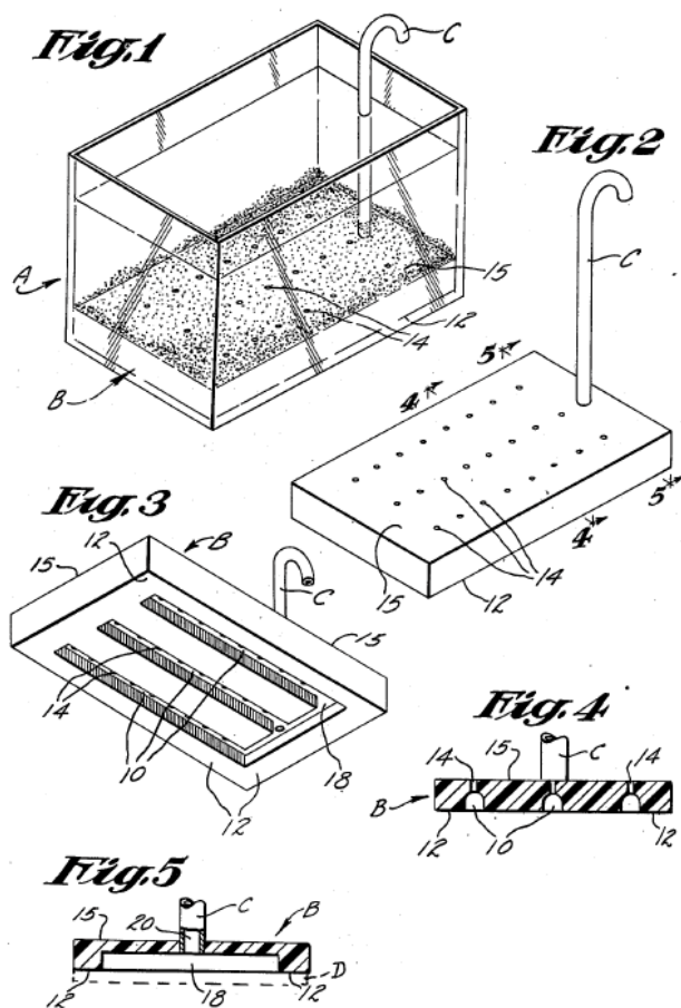
Figure 184: Albert J. Schwartz and Samuel H. Barbour's undergravel filter, 1953.
