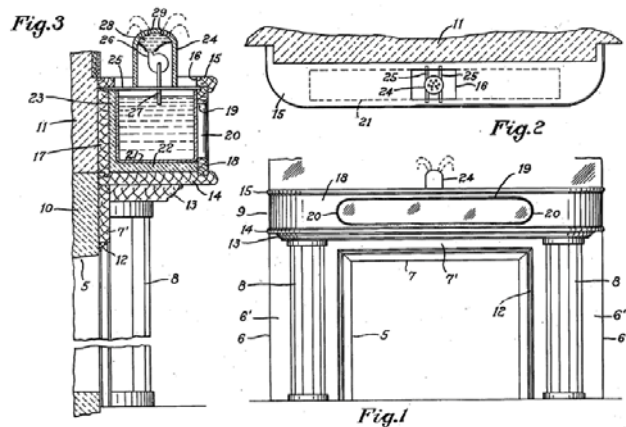
Figure 222: Alice J. Grossniklaus's fireplace mantle aquarium, 1950.
