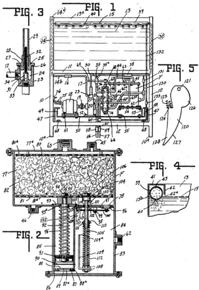
Figure 165: James F. Haldeman's aeration and filtration system, 1941.
