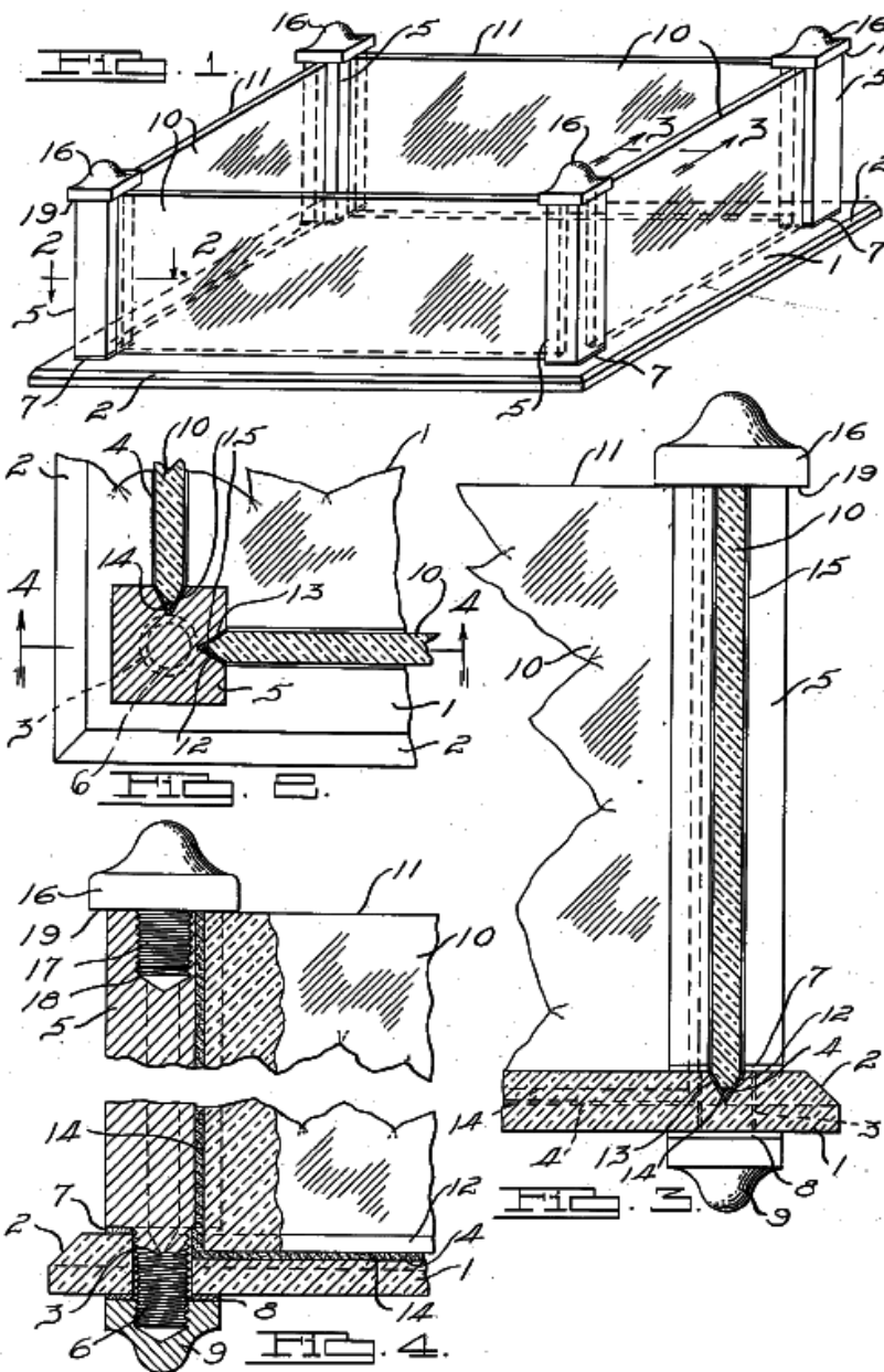
Figure 92: Alfred C. Schoepfer's V-groove, glass construction, 1933.
