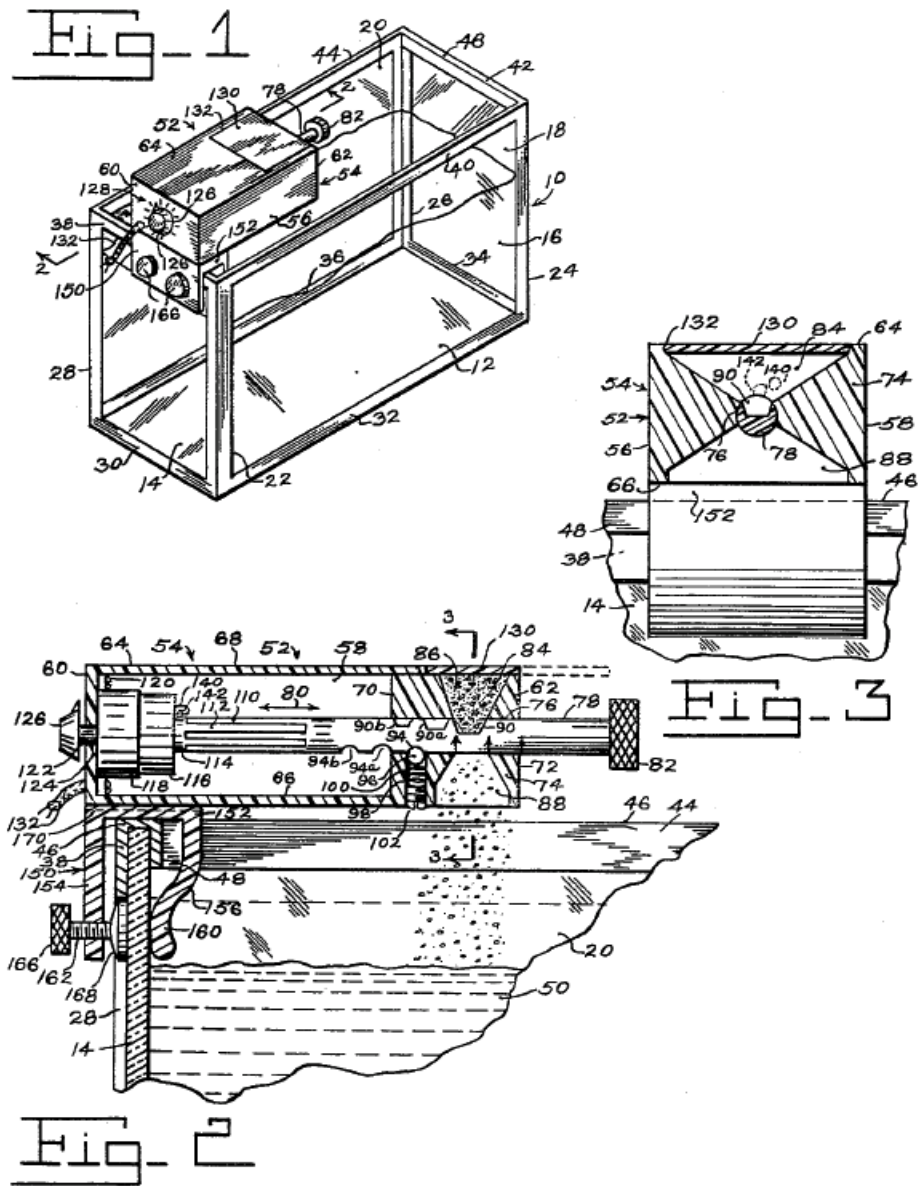
Figure 200: Seymour Smolin's notched shaft automatic feeding device, 1957.
