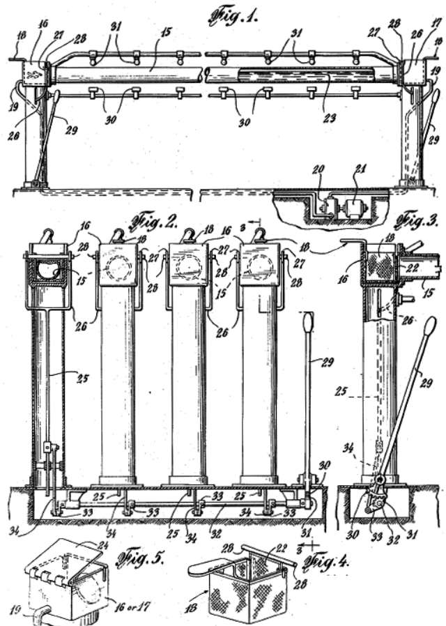
Figure 110: Irving I. Levenstein's fish race track, 1938.
