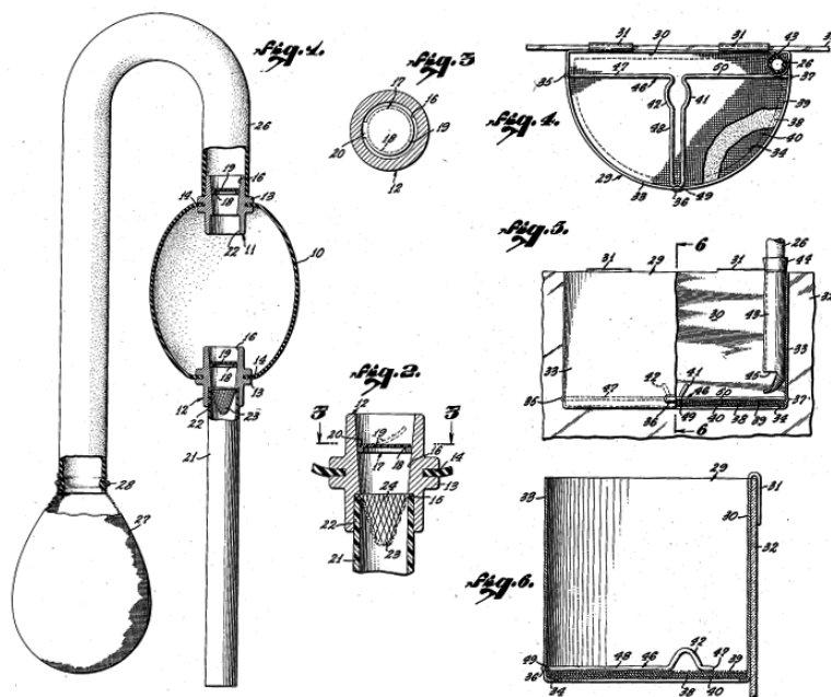
Figure 181: Clyde E. Hutchinson's cleaning device, 1954.
