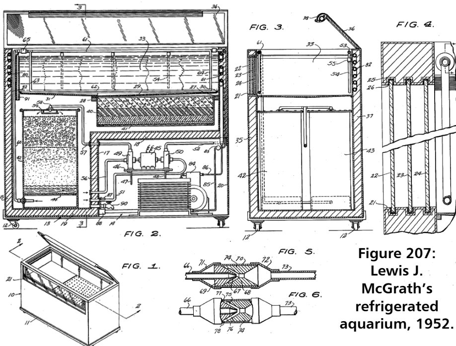
[Figure 207, Refrigerated Display Tank, Number 2594474 ] A refrigerated display tank patent for ma-
