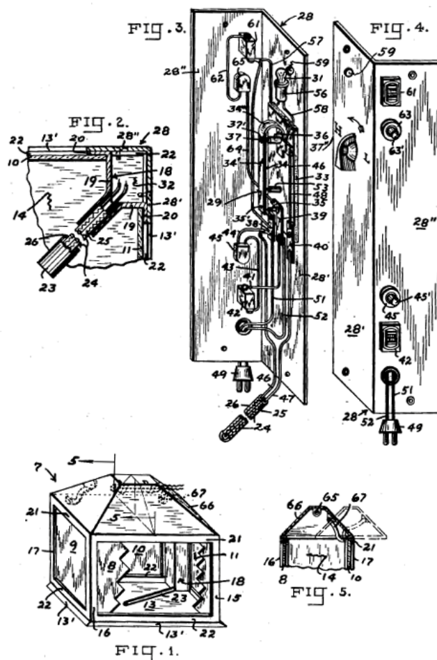
Figure 191: Andrew Mahle's integral heating design, 1951.
